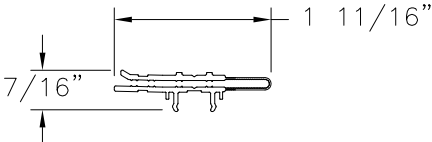
STORM CONNECT 1 PIECE VINYL, BY MUHLER
