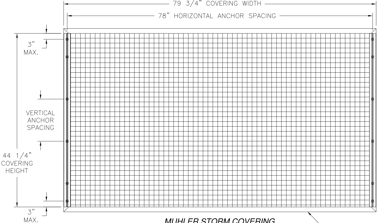
MUHLER STORM COVERING HORIZONTAL INSTALLATION REFER TO SHEET 4 FOR MULTIPLE UNIT PROTECTION
